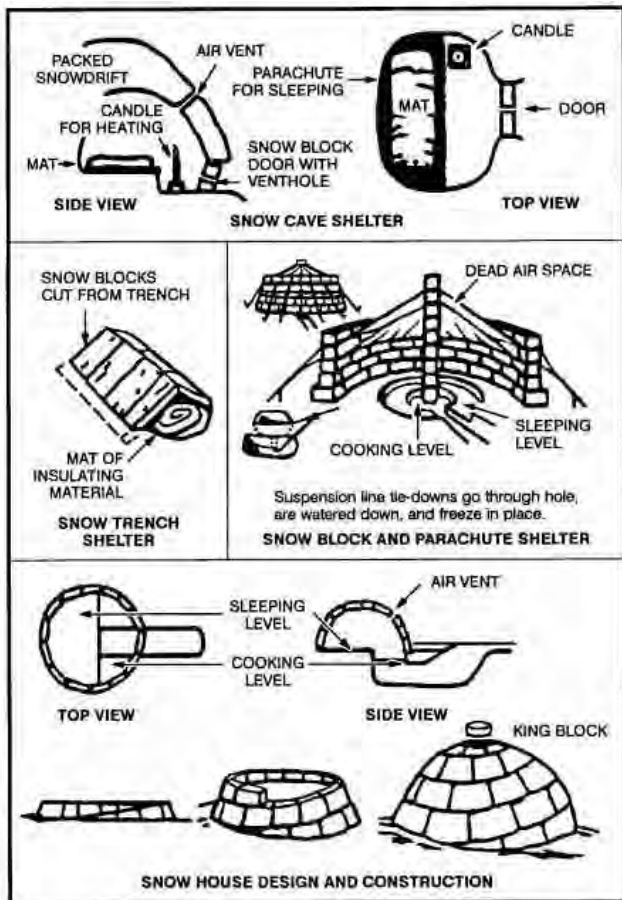
Figure 15-4. Snow houses.
