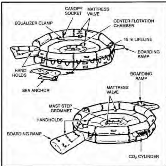
Figure 16-15. Twenty-man raft.
