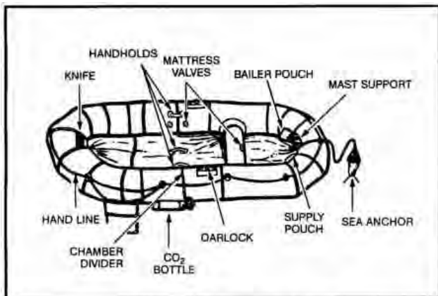
Figure 16-12. Seven-man raft.
