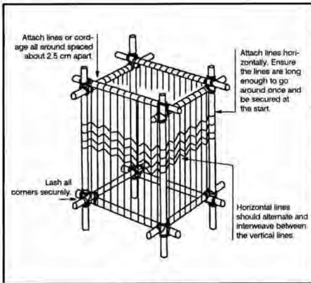
Figure 12-10. Square pack.
