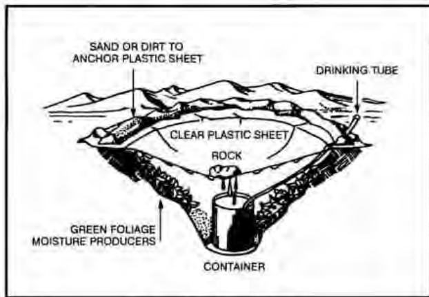
Figure 6-7. Belowground still.
