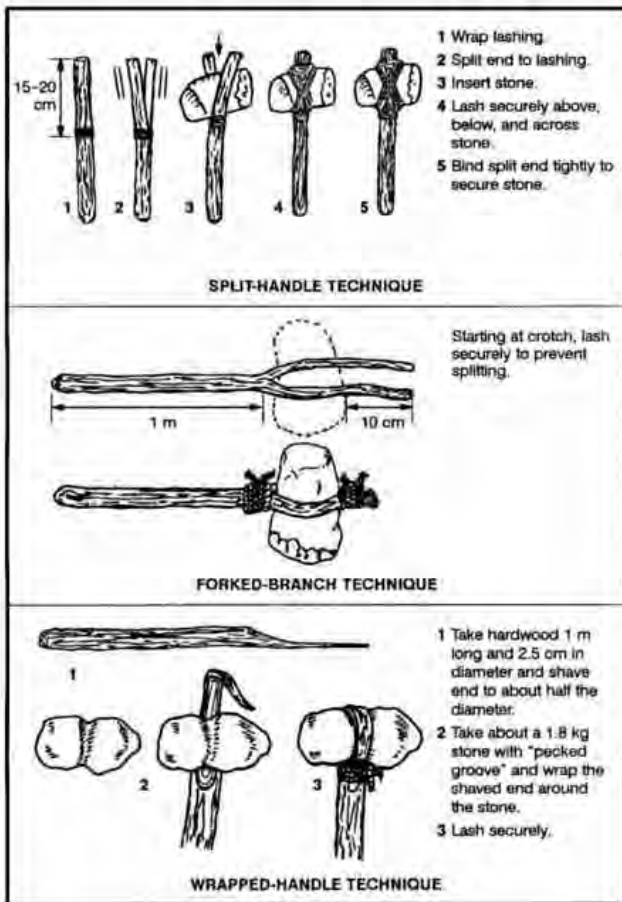
Figure 12-1. Lashing clubs.
