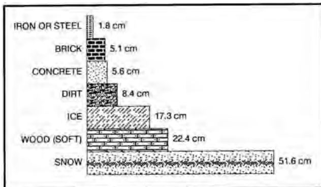
Figure 23-1. Thickness of materials to reduce gamma radiation.
